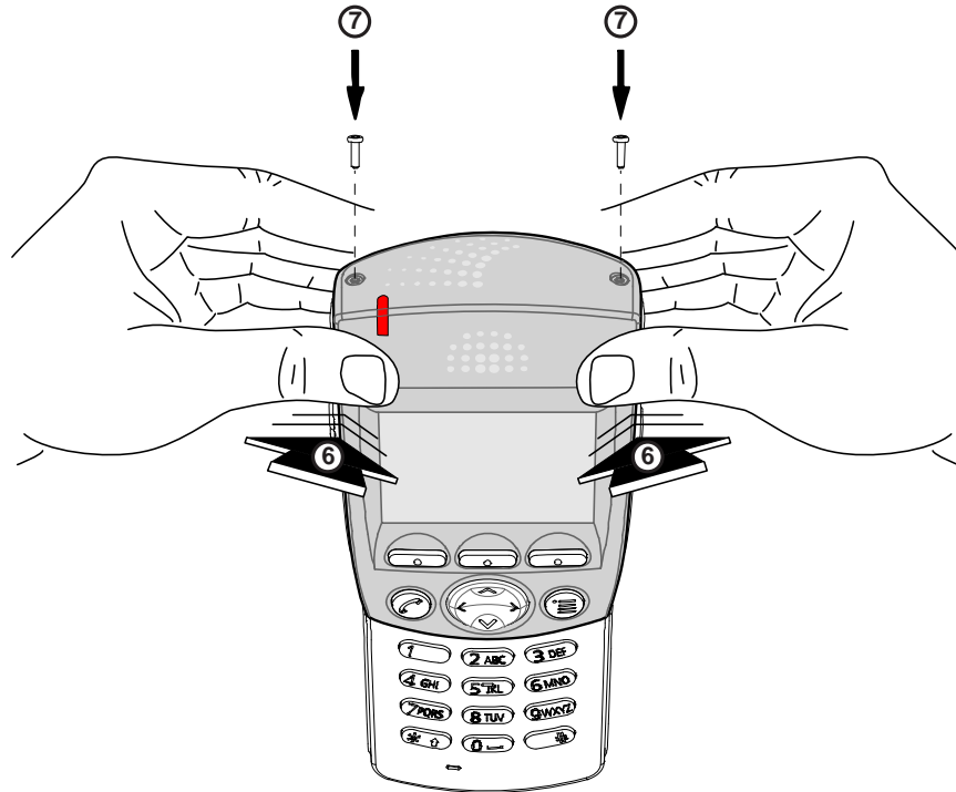
Figure 5 – Fasten the top front with two screws, utilizing a T6 torque driver set to 14Ncm.
