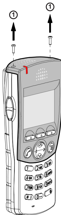
Figure 1 – Release the two screws at top on the handset.
